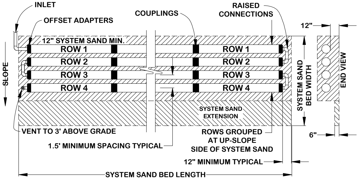
Rows grouped at high contour for sloping beds
