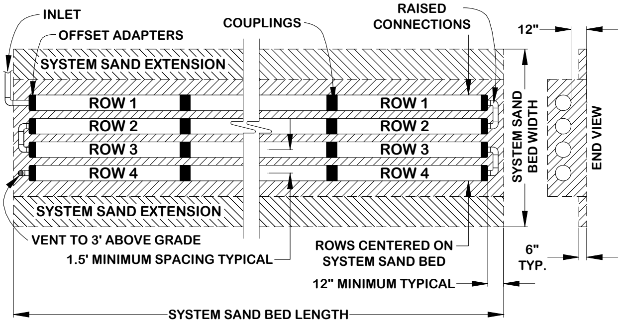
Rows centered on System Sand for level beds
